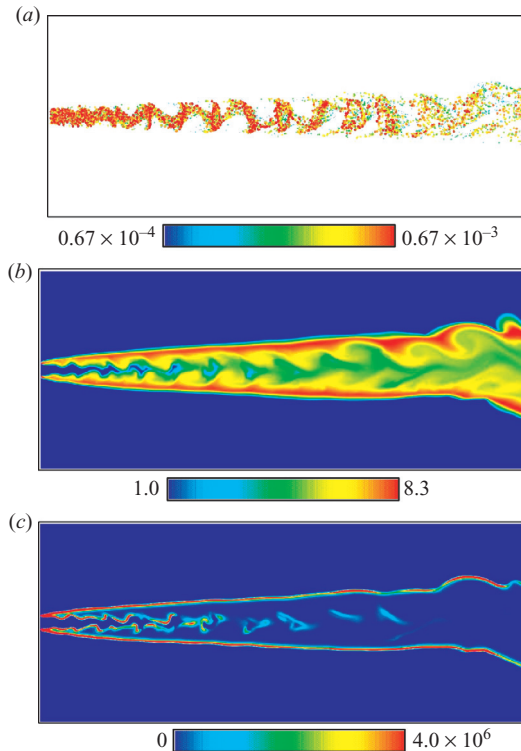
FIGURE 14. An instantaneous features of spray flame obtained in the case of LAR: (a) droplet distribution and diameter d_d^* , (b) gaseous temperature T^* and (c) reaction rate \dot{m}_v^* .
