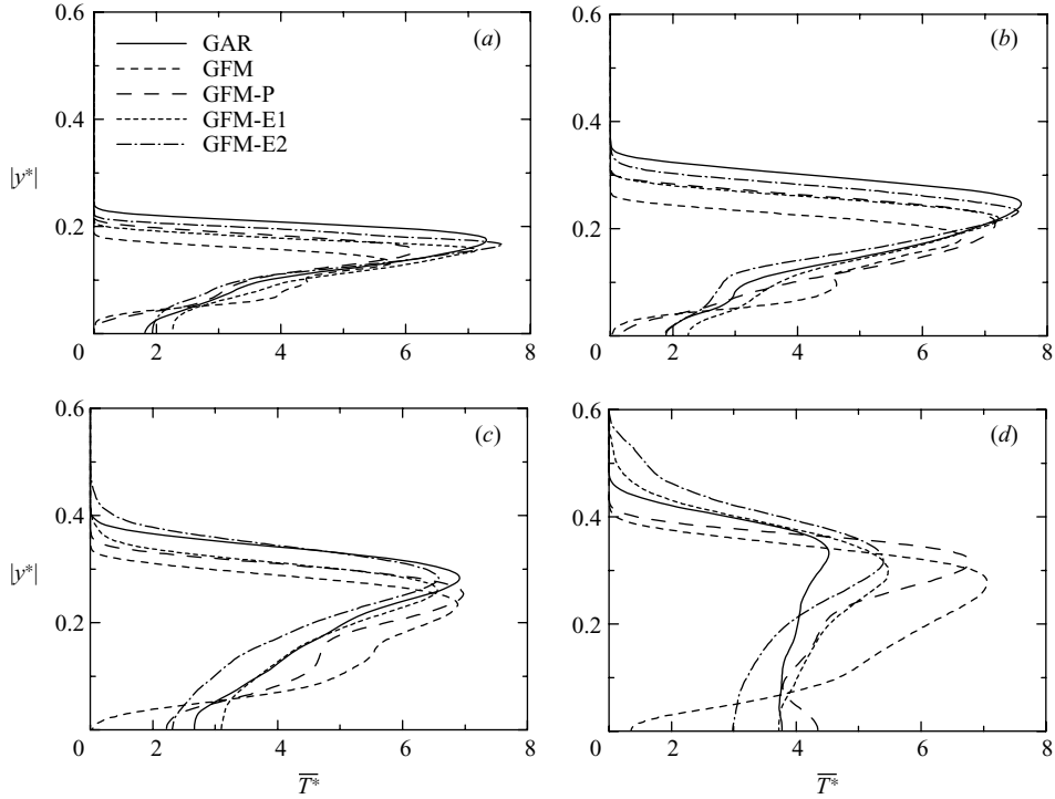
FIGURE 10. Comparison of spanwise profile of time-averaged gaseous temperature \overline{T^*} at four streamwise locations. (a) x^* = 1.0 , (b) x^* = 2.0 , (c) x^* = 3.0 and (d) x^* = 4.0 .
