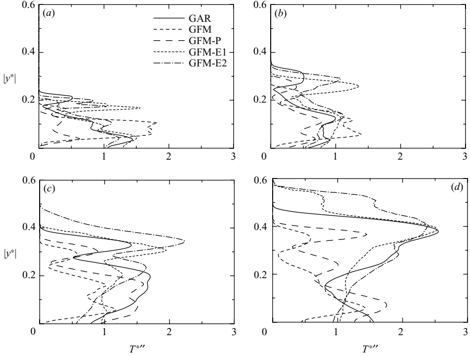
FIGURE 11. Comparison of spanwise profile of r.m.s. of gaseous temperature T^{*''} at four streamwise locations. (a) x^* = 1.0 , (b) x^* = 2.0 , (c) x^* = 3.0 and (d) x^* = 4.0 .
