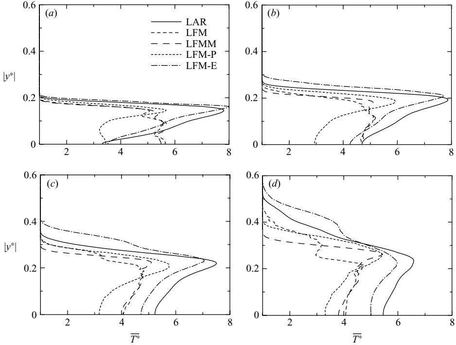
FIGURE 22. Comparison of spanwise profile of time-averaged gaseous temperature \overline{T^*} at four streamwise locations. (a) x^* = 1.0 , (b) x^* = 2.0 , (c) x^* = 3.0 and (d) x^* = 4.0 .
