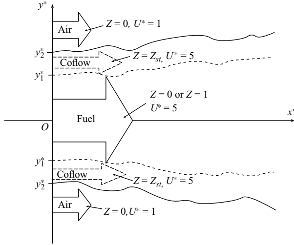
FIGURE 4. Schematic of computational domain and inlet conditions.
