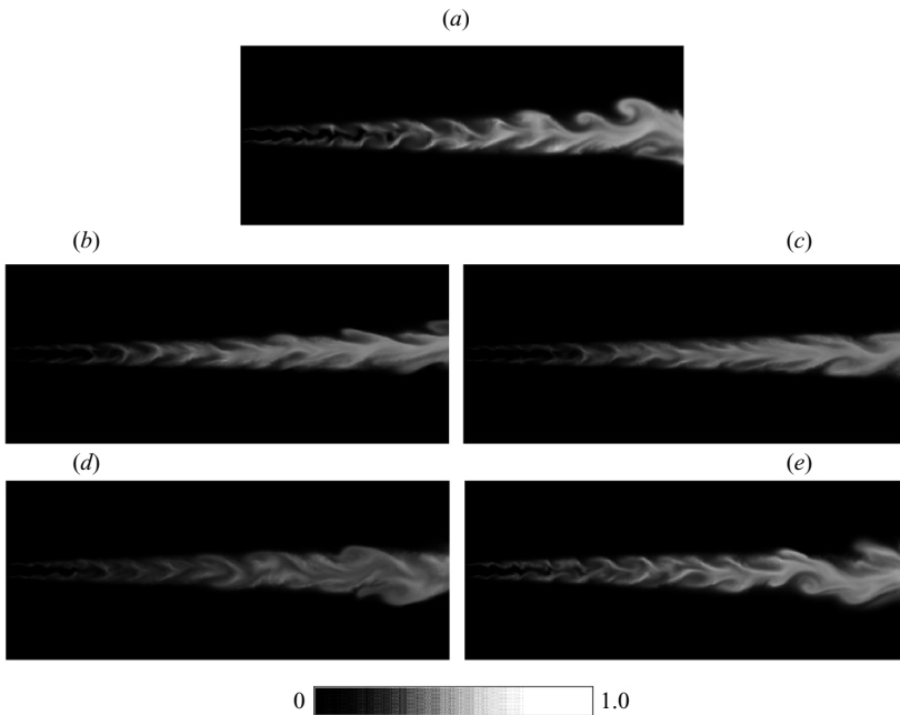
FIGURE 19. Comparison of instantaneous distribution of mixture fraction Z . (a) LAR, (b) LFM, (c) LFMM, (d) LFM-P and (e) LFM-E.
